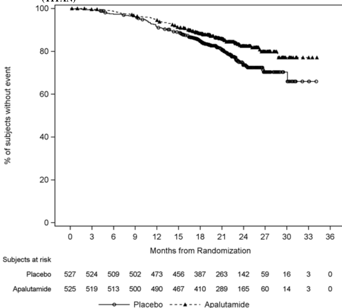
Figure 1: Kaplan-Meier Plot of Overall Survival (OS); Intent-to-treat mHSPC Population (TITAN)
